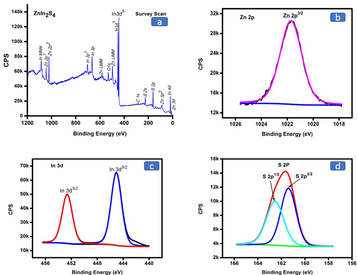
Fig. 2 XPS spectra of ZnIn 2 S 4 thin films fabricated on FTO at 500 °C using toluene solution of precursor (1) and (2) (a) Survey scan (b) Zn 2p 3/2 (c) In 3d 5/2 and (d) S 2p.
